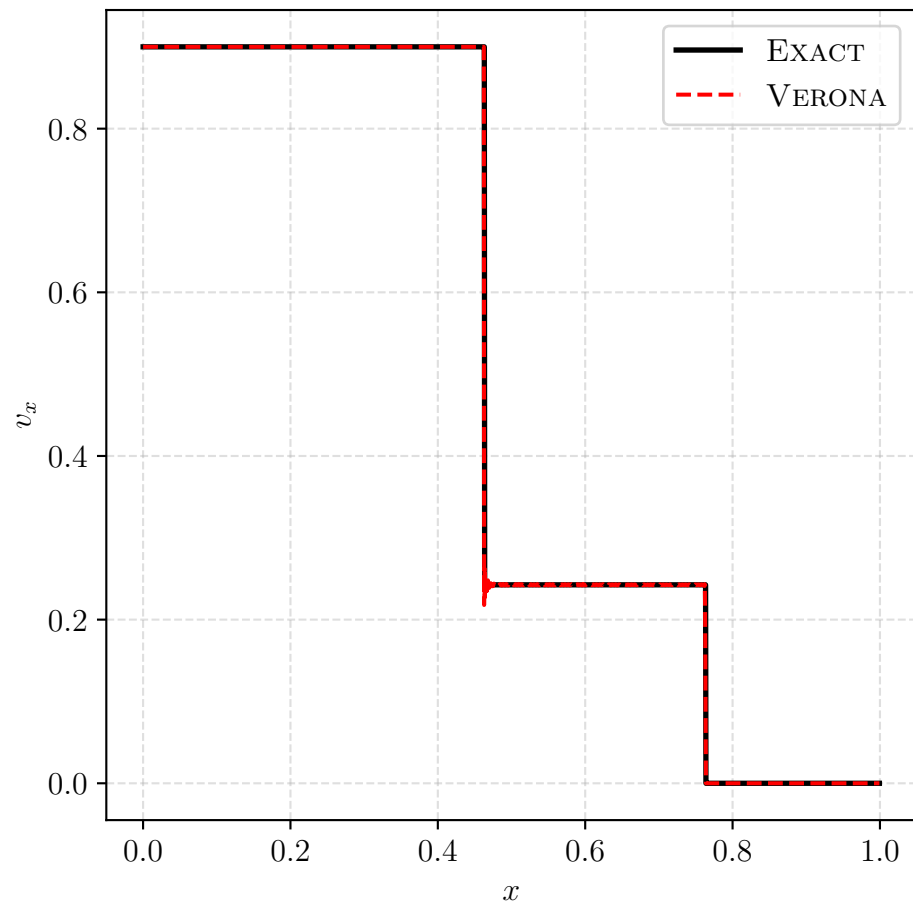
Shock Tube III
